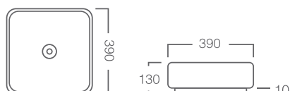
Encore 390 – Above Counter Basin Product Code: E390 (White) 390mm x 390mm x 130mm
