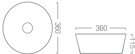
ASTER NEW - SEMI INSET BASIN
